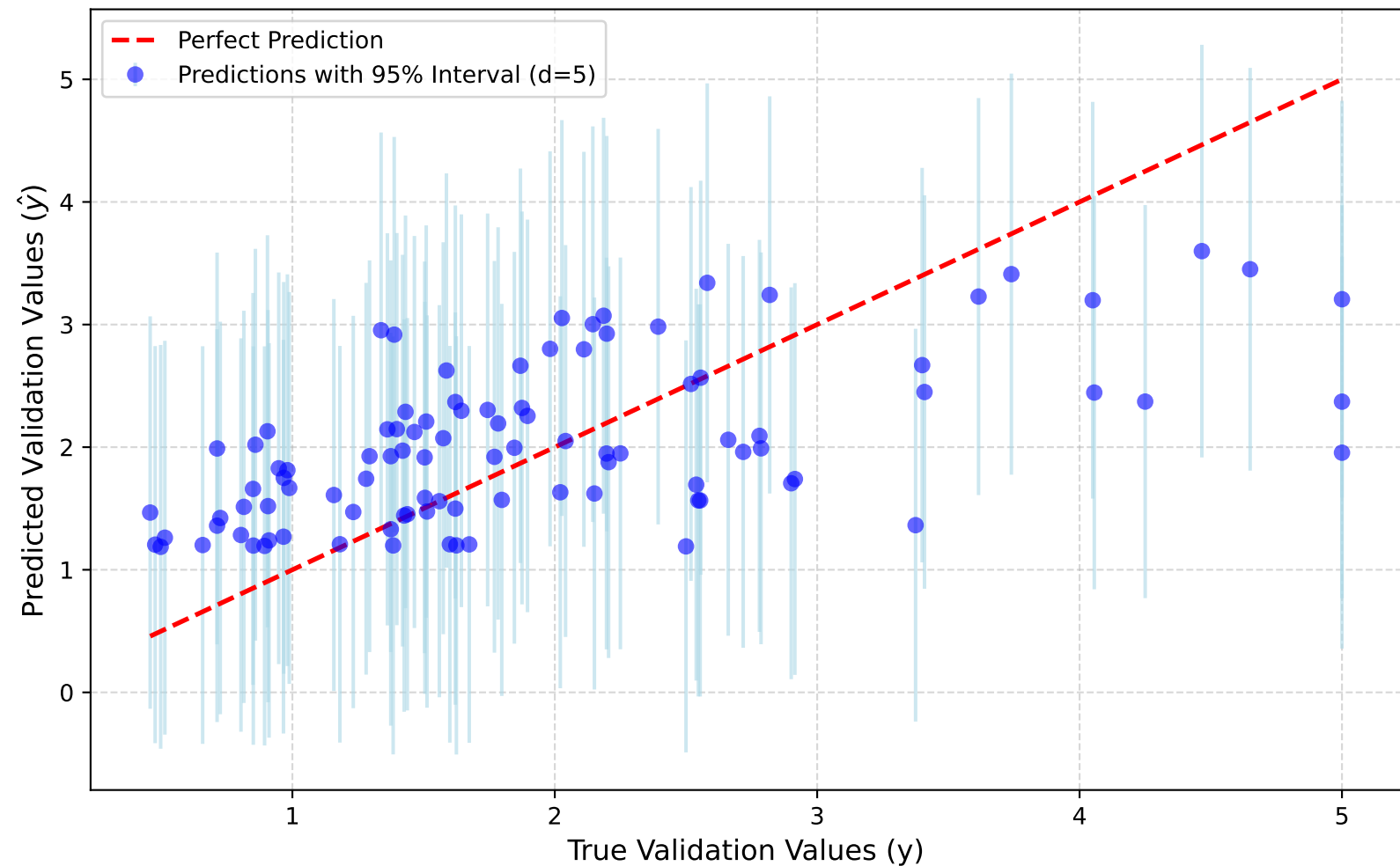
True vs. Predicted Values with 95% Prediction Intervals (d=5)
